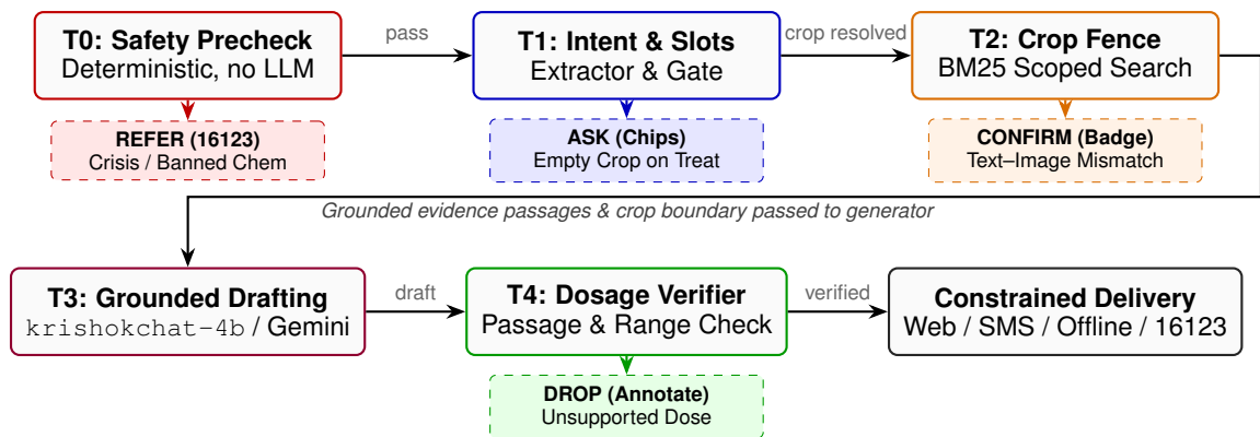
Figure 1: KrishokTech inserts explicit control points before and after generation. Each of the five stages can end a turn in a farmer-visible state: REFER at T0, ASK at T1, CONFIRM at T2, or DROP at T4.
